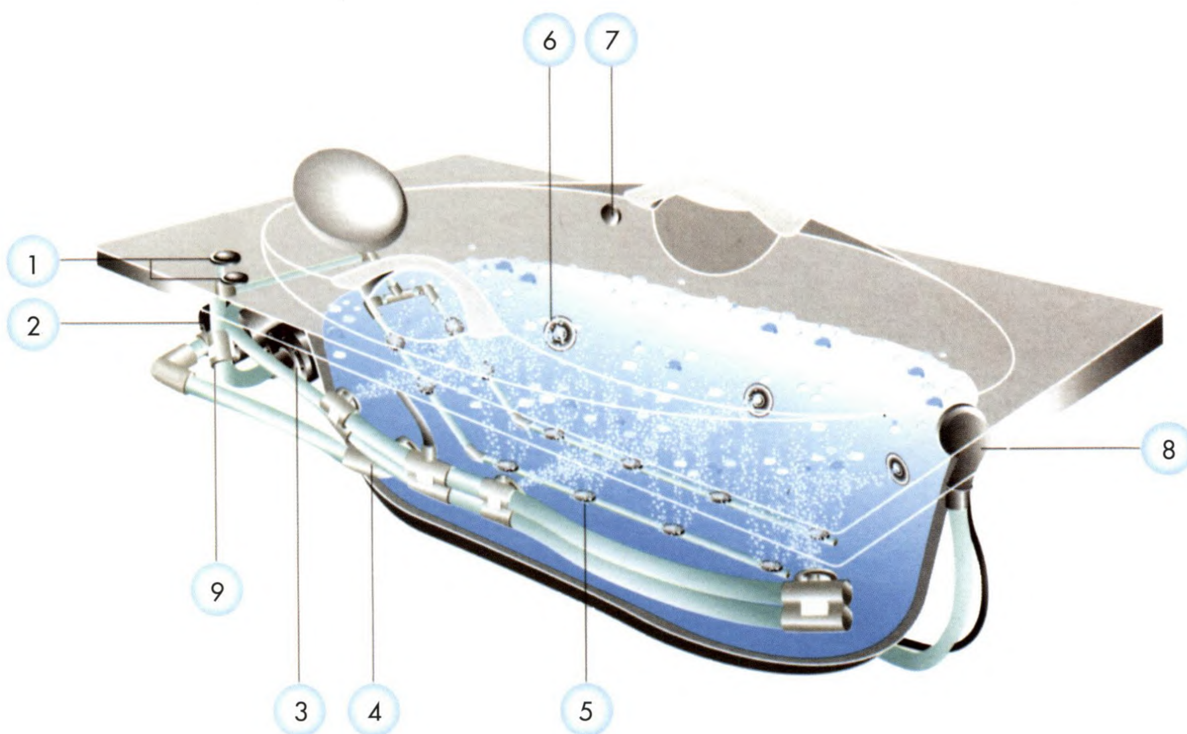
WHIRLPOOL SYSTEM
